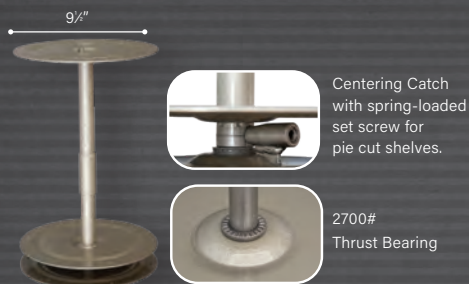
SIGNATURE PRO HARDWARE DETAIL
